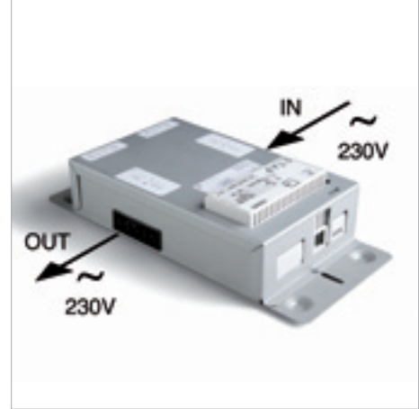
webref. SC027A2 Control unit
