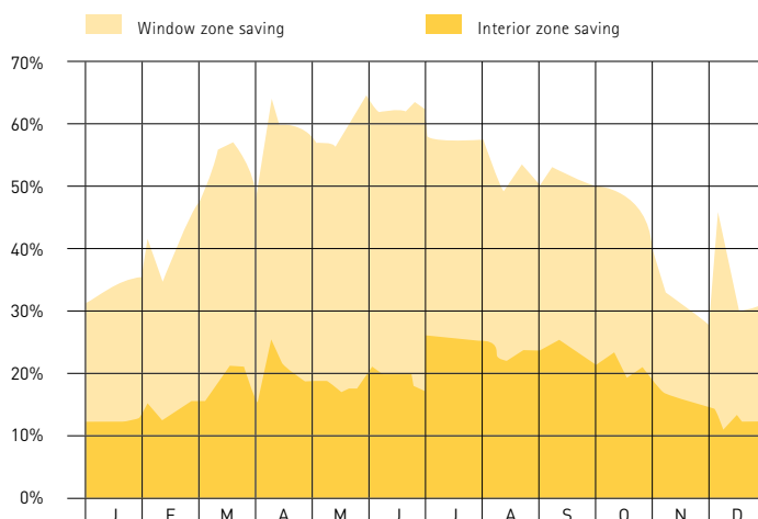
Energy saving of a luminaire with ELS. Potential energy savings are greatest during the summer months.
